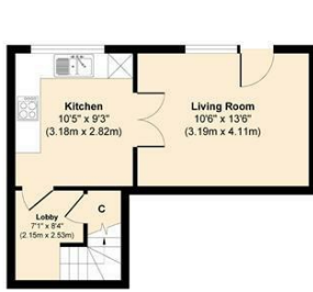
Lower Ground Floor Approximate Floor Area 302 sq. ft (28.04 sq. m)
